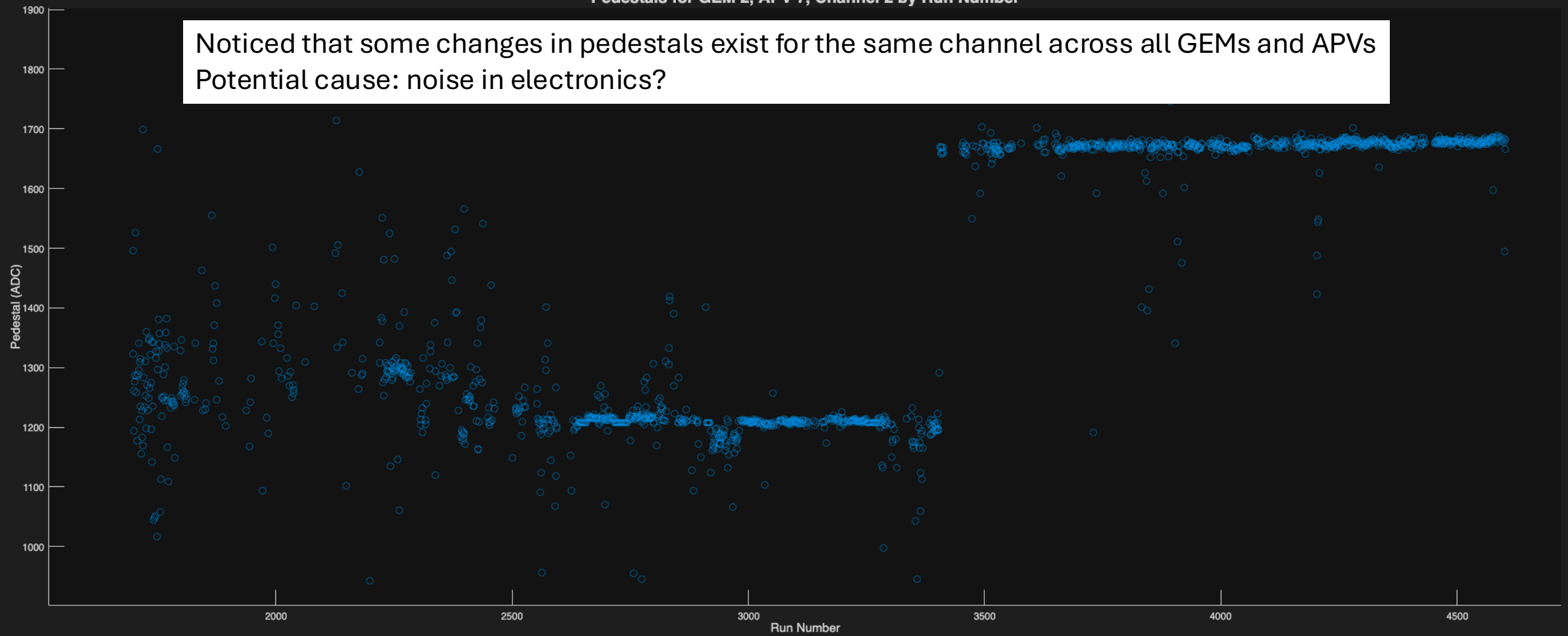
Pedestals for GEM 2, APV 7, Channel 2 by Run Number
